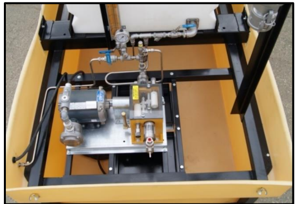
Example Tubing for BR4300 with PRV
